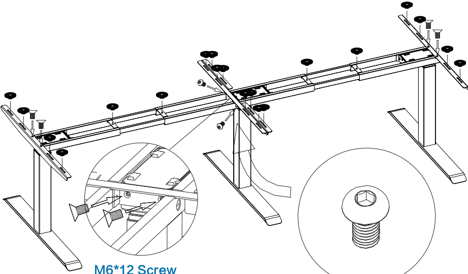
M6*12 Screw
